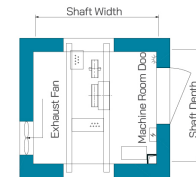
Machine Room Layout
