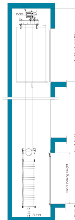
Shaft Vertical View
