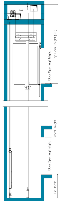
Shaft Vertical View
