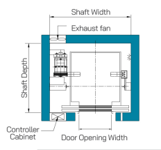
Shaft Head Layout
