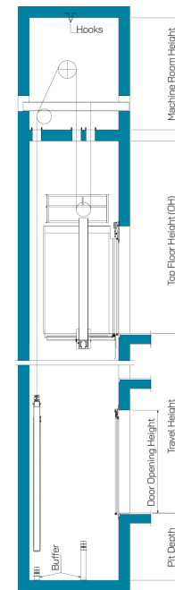
Shaft Vertical View
