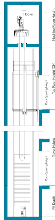
Shaft Vertical View
