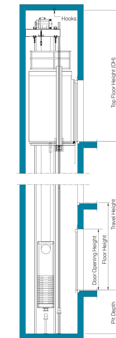
Shaft Vertical View
